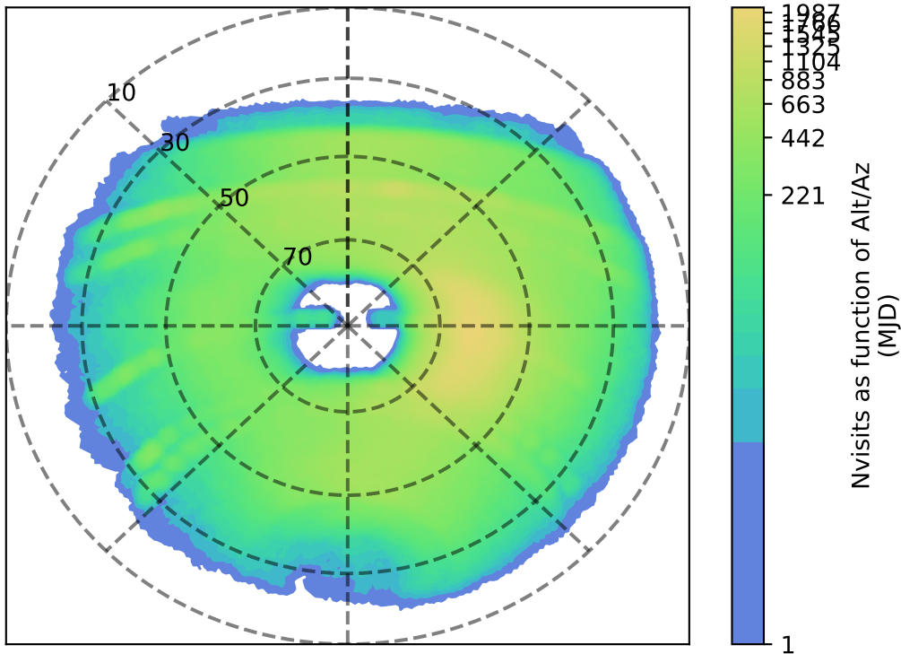
baseline_v3.4_10yrs y: Nvisits as function of Alt/Az
