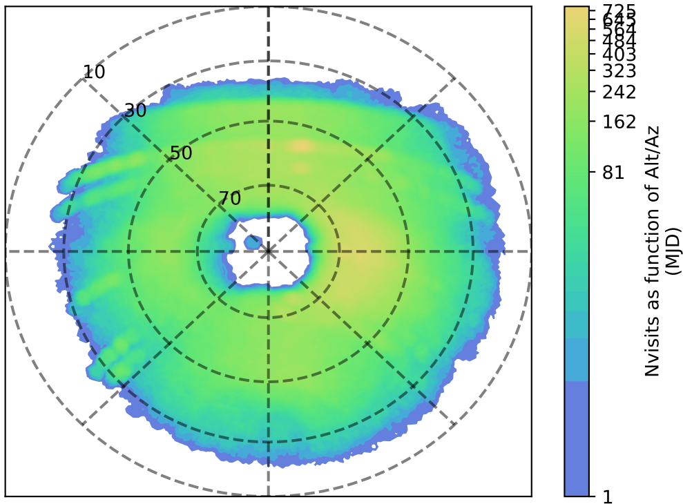
baseline_v3.4_10yrs u: Nvisits as function of Alt/Az
