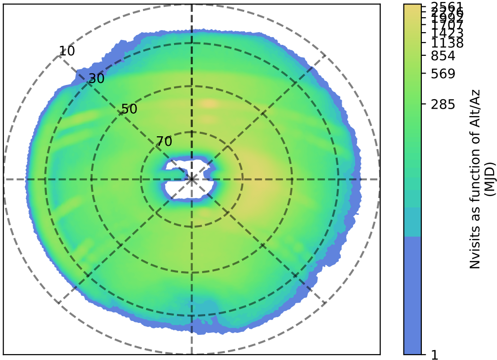
baseline_v3.4_10yrs r: Nvisits as function of Alt/Az
