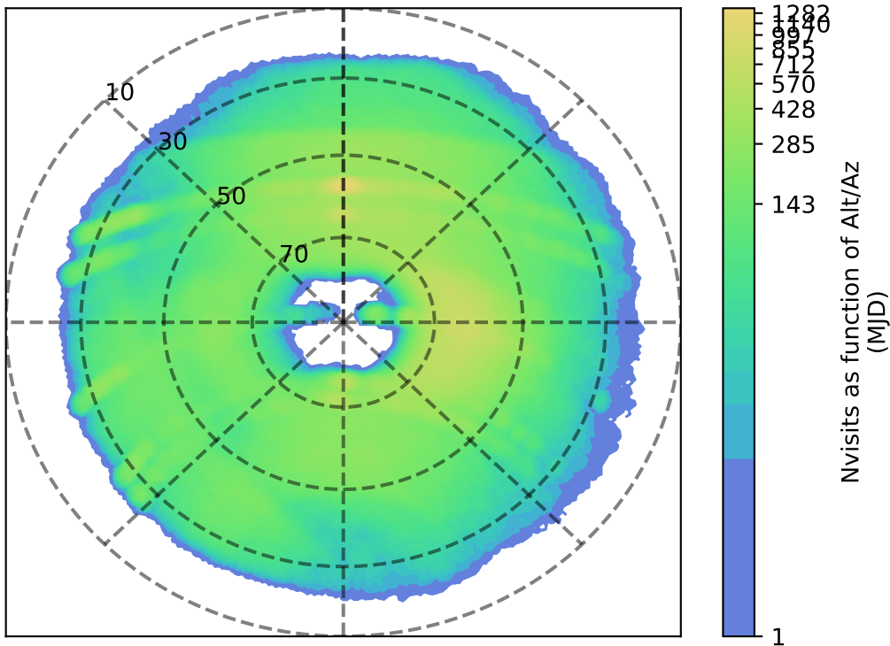
baseline_v3.4_10yrs g: Nvisits as function of Alt/Az
