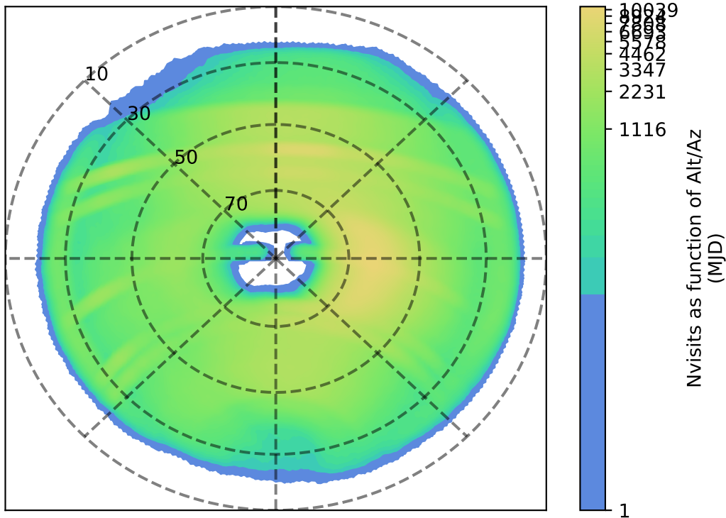
baseline_v3.4_10yrs : Nvisits as function of Alt/Az
