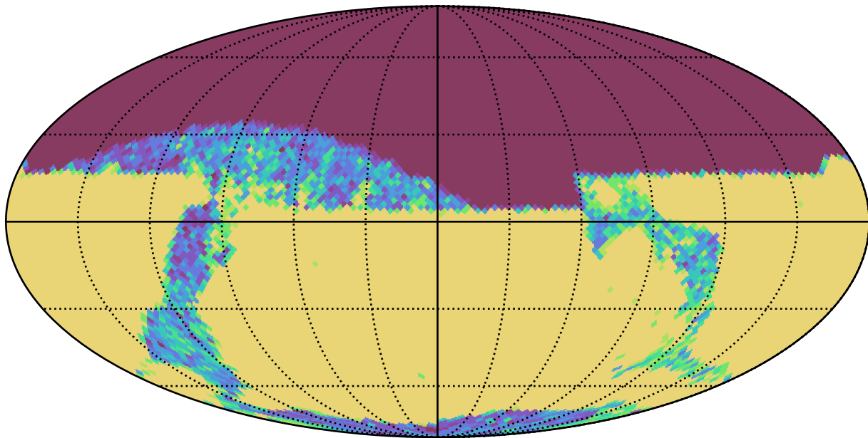
baseline_v3.4_10yrs z and night < 365: N year 1
