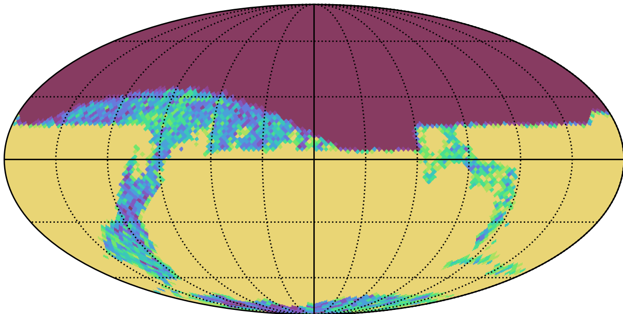
baseline_v3.4_10yrs r and night < 365: N year 1
