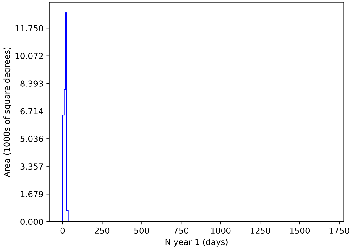
baseline_v3.4_10yrs r and night < 365: N year 1
