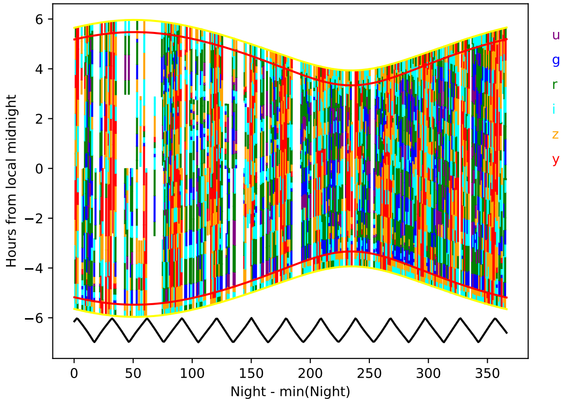
baseline_v3.4_10yrs year 9-10: Hourglass
