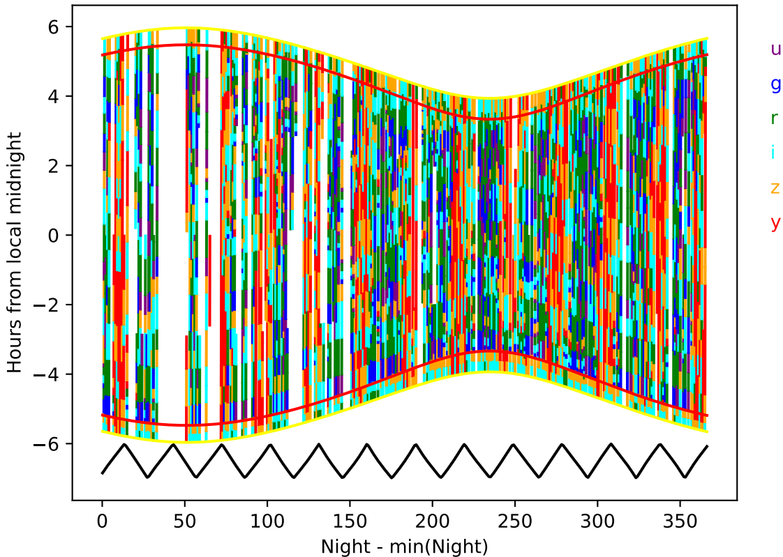
baseline_v3.4_10yrs year 8-9: Hourglass
