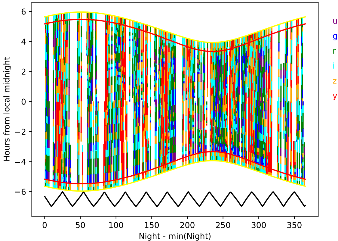
baseline_v3.4_10yrs year 7-8: Hourglass
