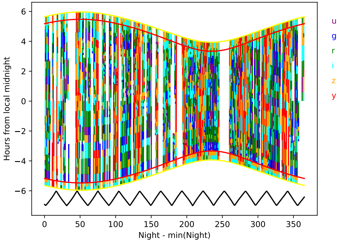
baseline_v3.4_10yrs year 5-6: Hourglass
