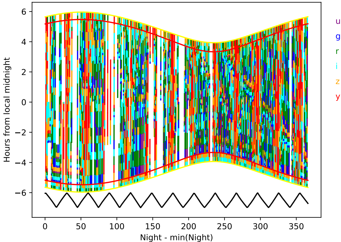
baseline_v3.4_10yrs year 1-2: Hourglass
