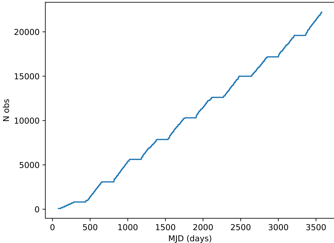
baseline_v3.4_10yrs note like DD:XMM_LSS%: Cumulative
