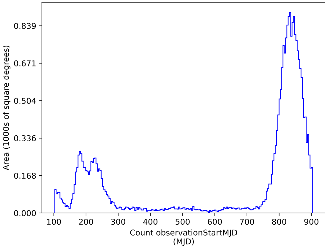
baseline_v3.4_10yrs : Count observationStartMJD
