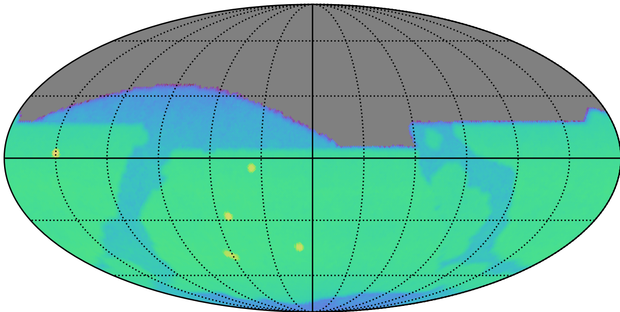
baseline_v3.4_10yrs z: CoaddM5
