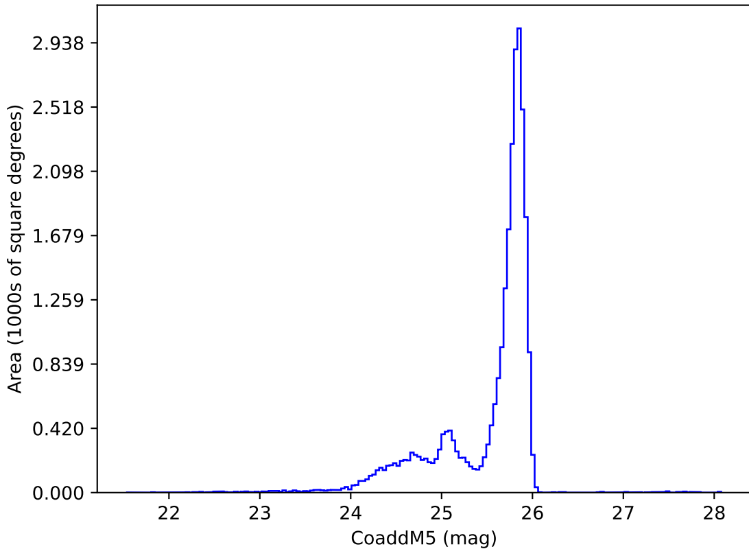
baseline_v3.4_10yrs z: CoaddM5
