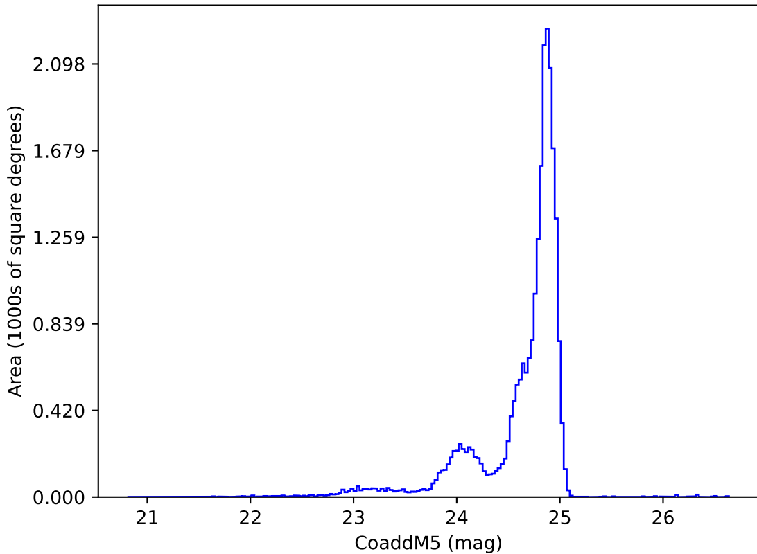
baseline_v3.4_10yrs y: CoaddM5
