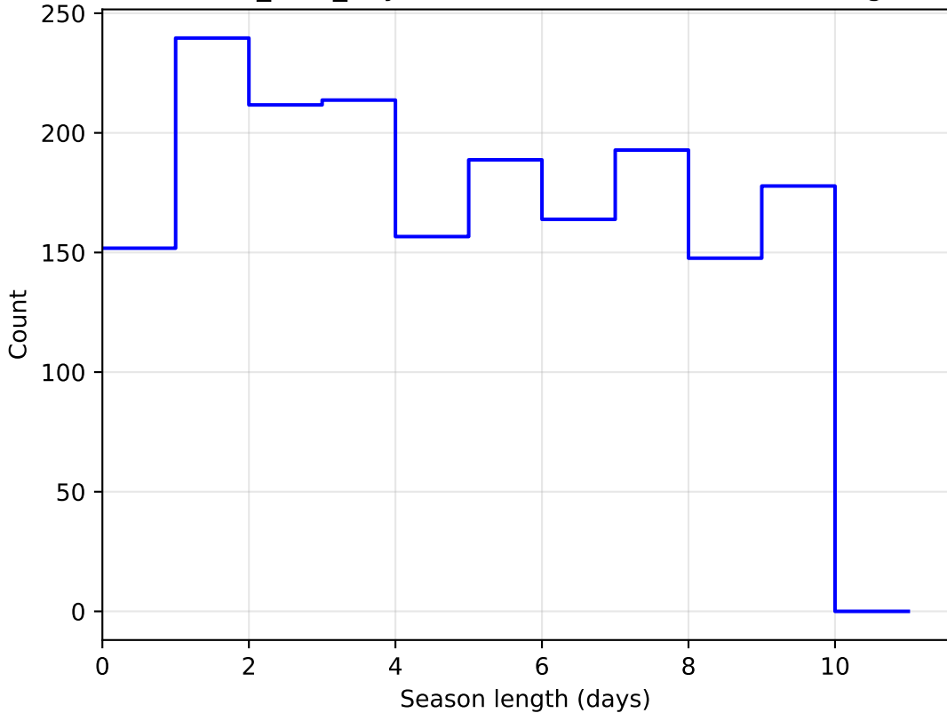
baseline_v3.4_10yrs DD:WFD all bands: SeasonLength
