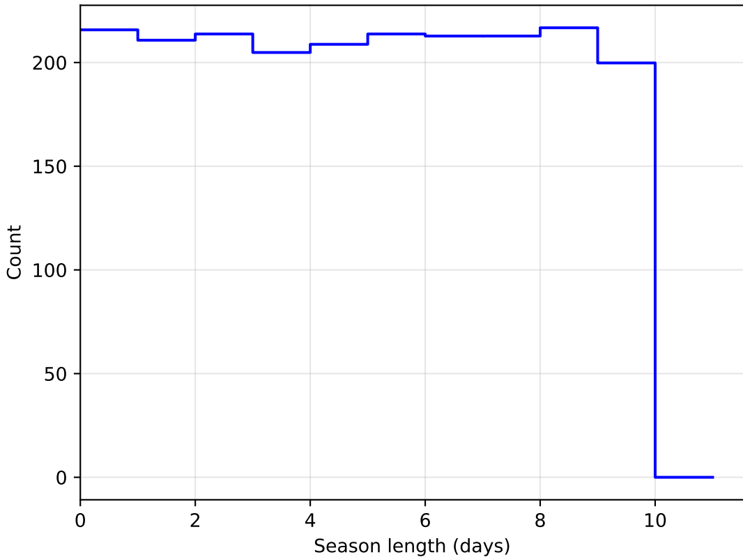
baseline_v3.4_10yrs DD:ECDFS all bands: SeasonLength
