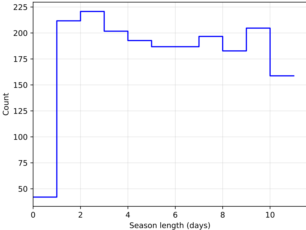
baseline_v3.4_10yrs DD: COSMOS all bands: SeasonLength
