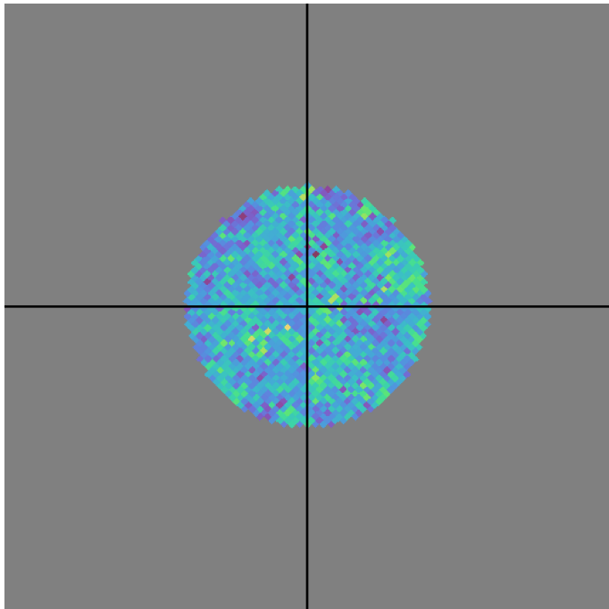
baseline_v3.4_10yrs DD:WFD all bands: SNSLMetric
