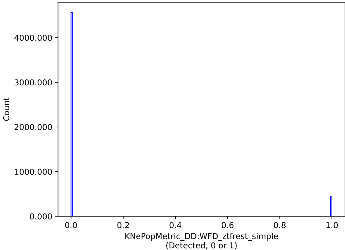
baseline_v3.4_10yrs DD:WFD: KNePopMetric_DD:WFD_ztfrest_simple
