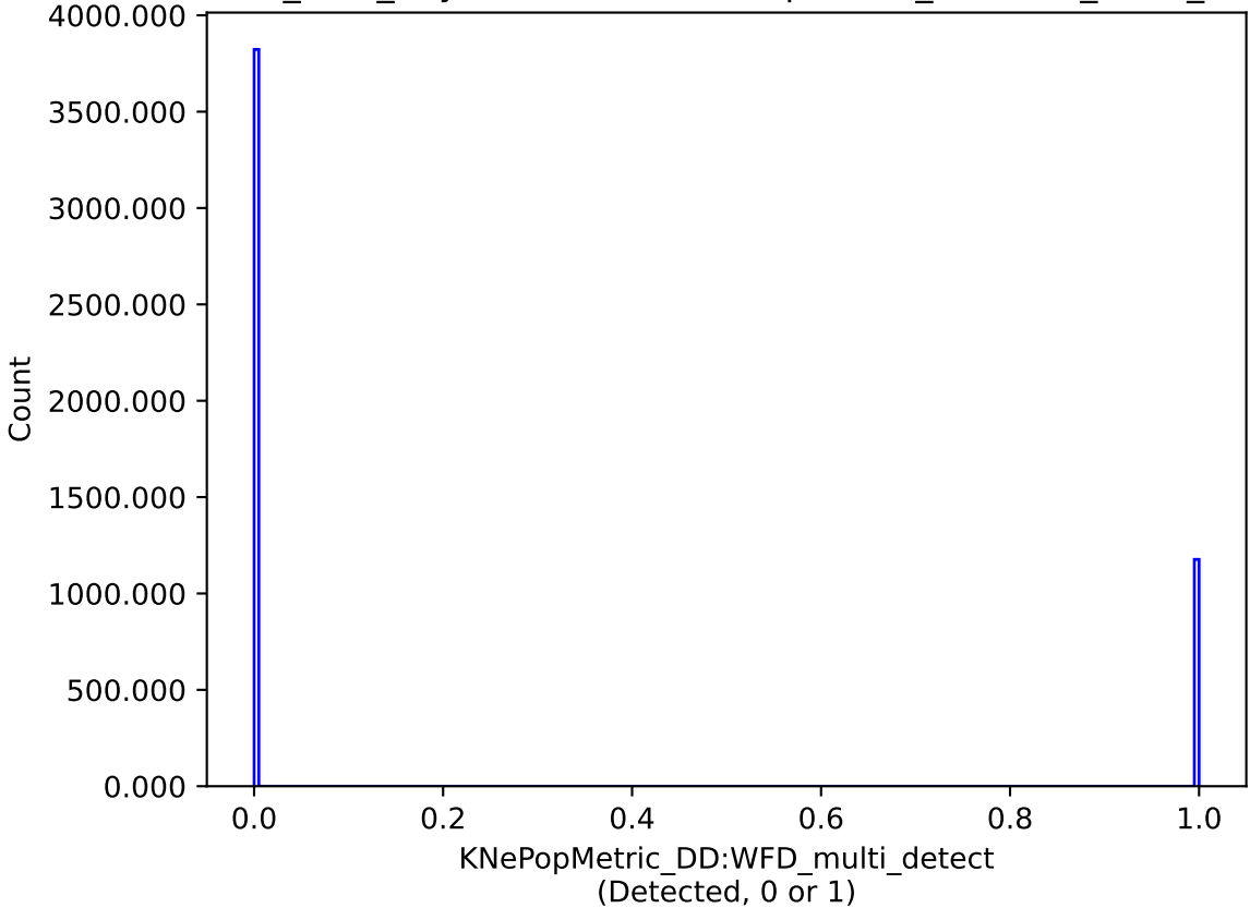
baseline_v3.4_10yrs DD:WFD: KNePopMetric_DD:WFD_multi_detect
