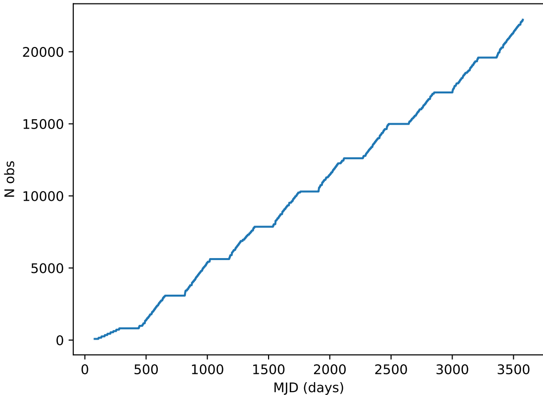
baseline_v3.4_10yrs all bands: DD:XMM_LSS Cumulative NVisits
