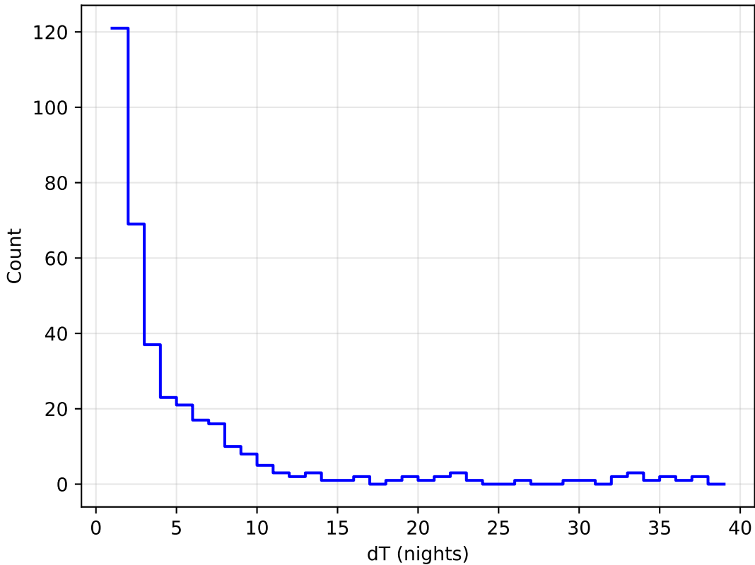
baseline_v3.4_10yrs all bands: DD:WFD Delta Nights Histogram
