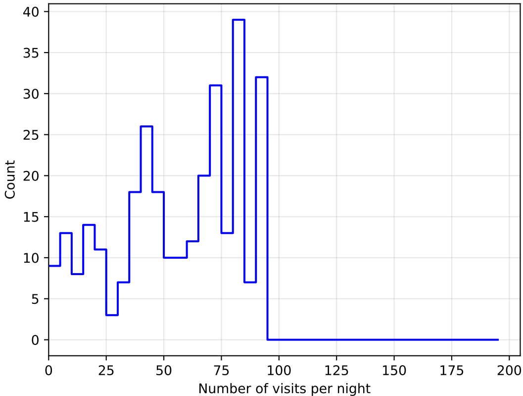
baseline_v3.4_10yrs all bands: DD:EDFS NVisitsPerNight
