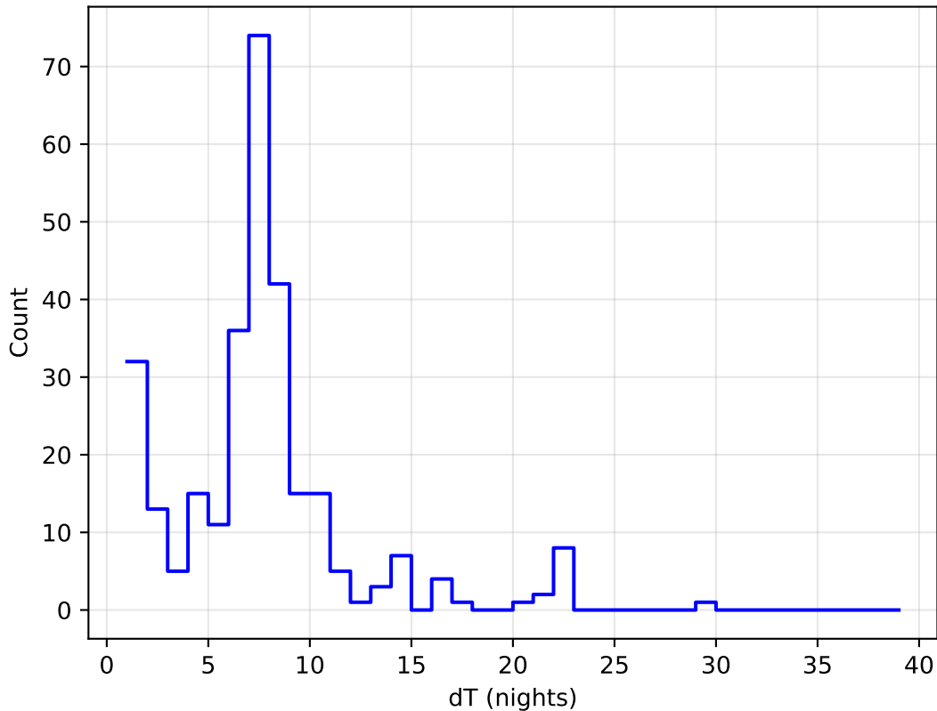
baseline_v3.4_10yrs all bands: DD:EDFS Delta Nights Histogram
