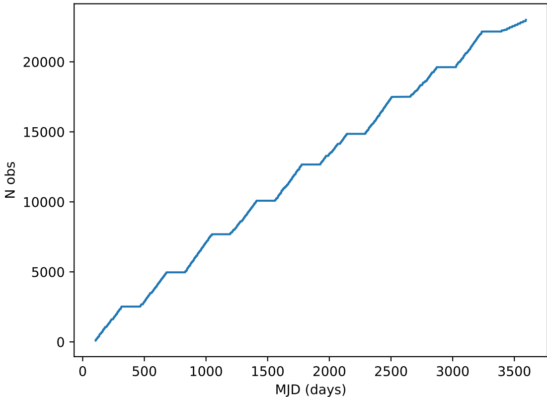
baseline_v3.4_10yrs all bands: DD:EDFS Cumulative NVisits
