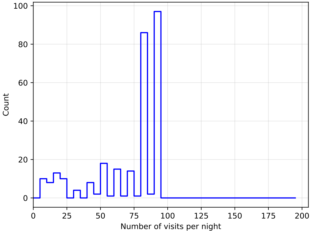
baseline_v3.4_10yrs all bands: DD:ECDFS NVisitsPerNight
