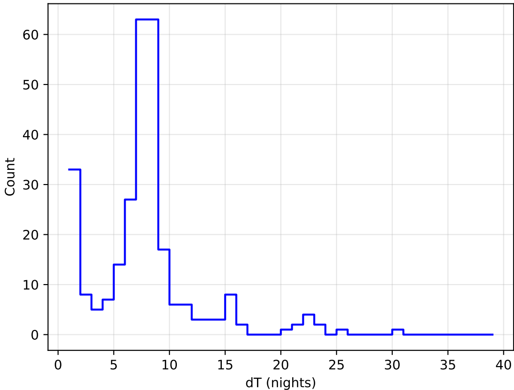
baseline_v3.4_10yrs all bands: DD:ECDFS Delta Nights Histogram
