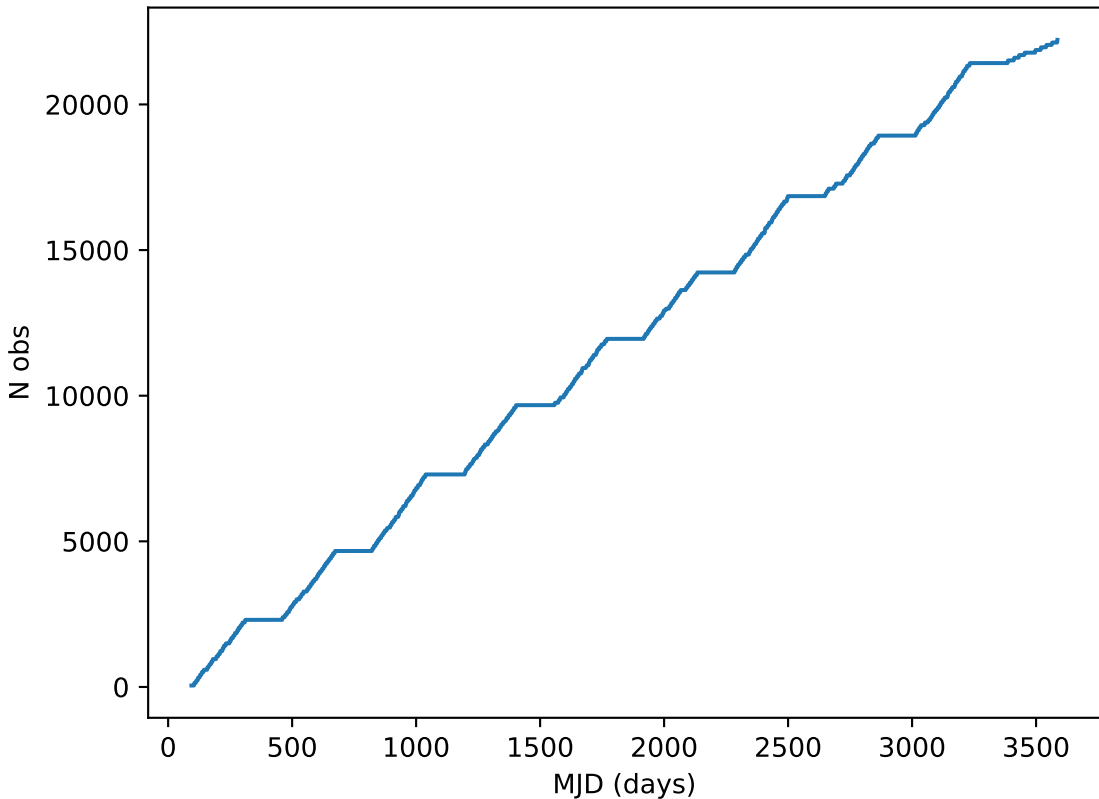
baseline_v3.4_10yrs all bands: DD:ECDFS Cumulative NVisits
