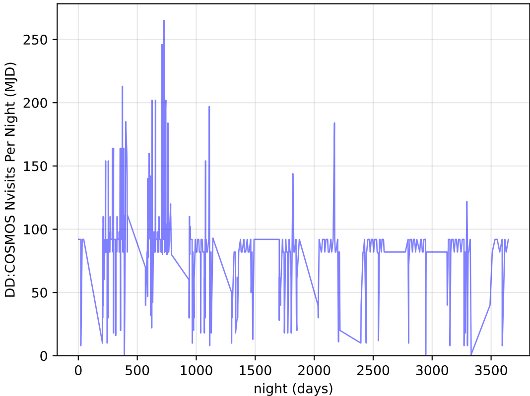
baseline_v3.4_10yrs all bands: DD:COSMOS Nvisits Per Night
