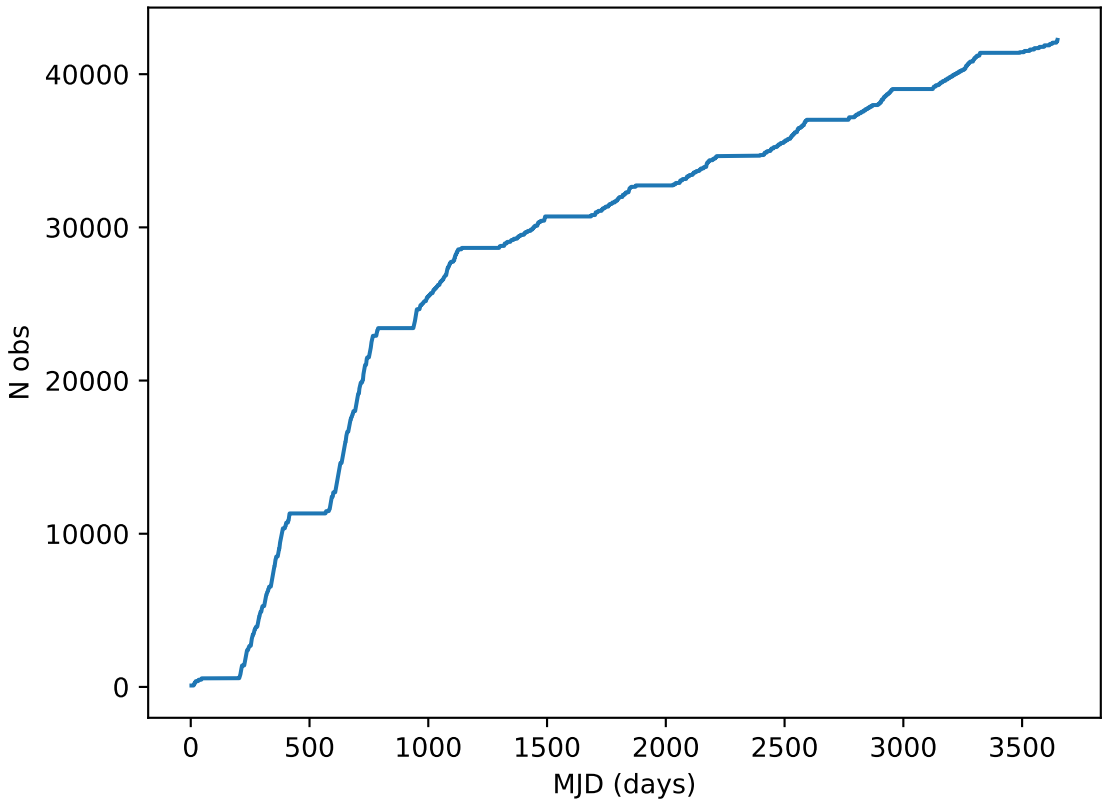
baseline_v3.4_10yrs all bands: DD:COSMOS Cumulative NVisits
