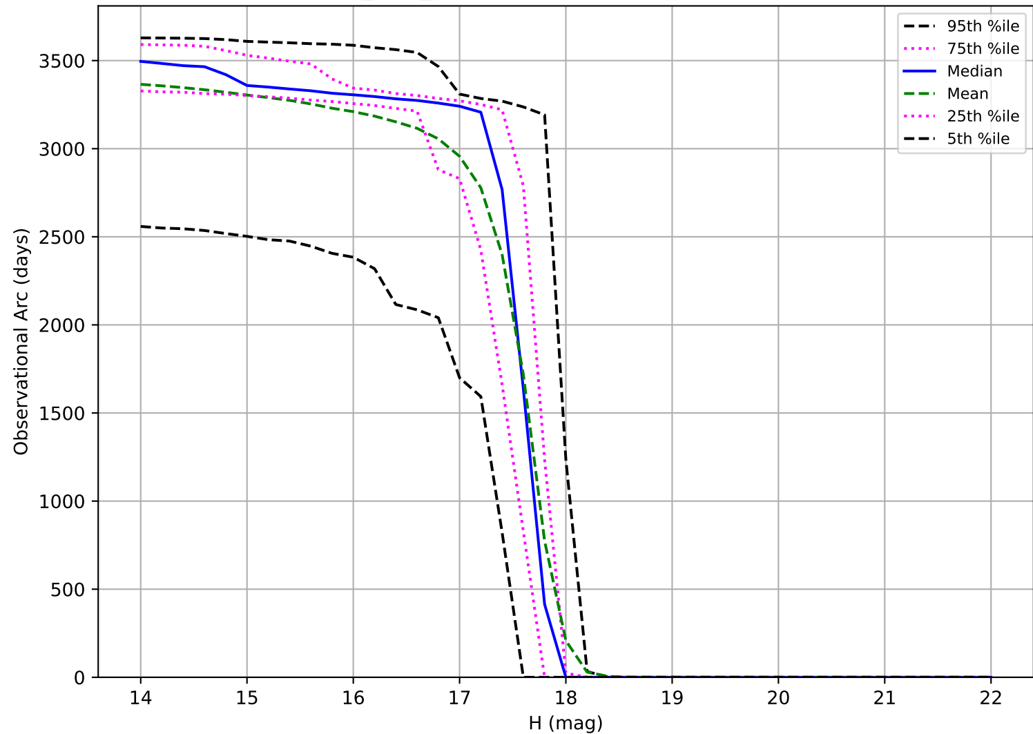
baseline_v3.3_10yrs: Observational Arc Length Trojan
