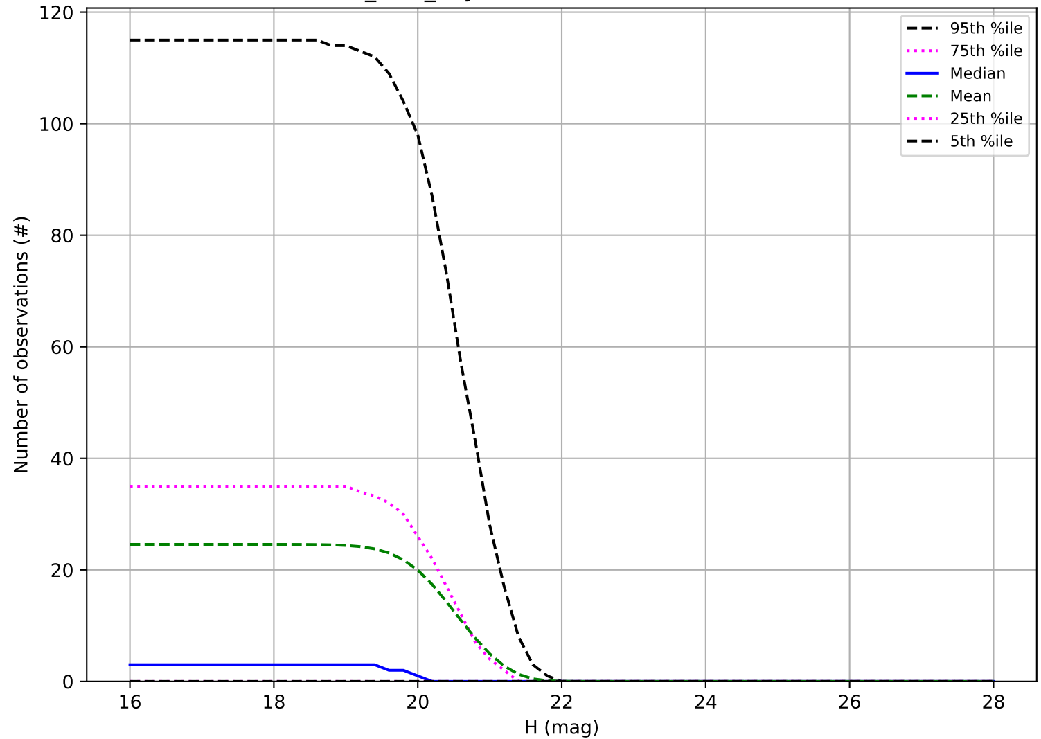
baseline_v3.3_10yrs: Number of observations Vatira
