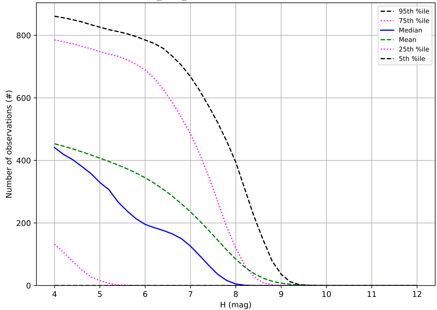
baseline_v3.3_10yrs: Number of observations TNO
