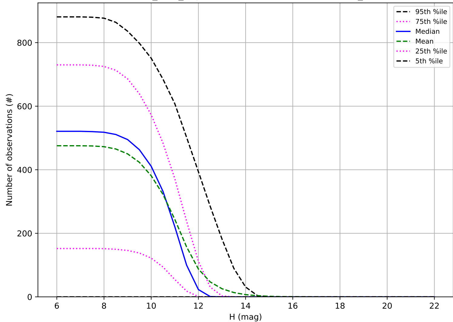
baseline_v3.3_10yrs: Number of observations OCC_r20
