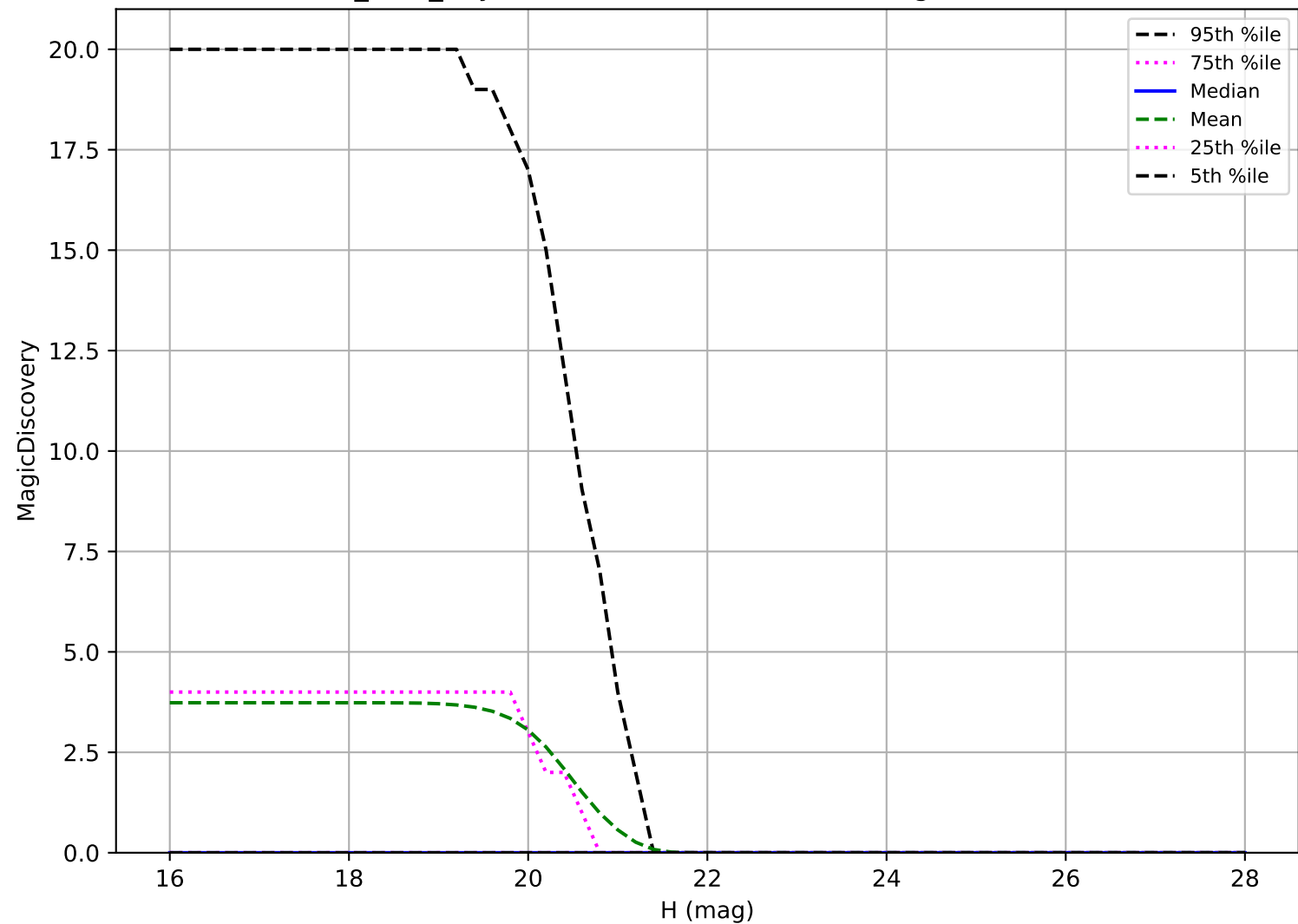
baseline_v3.3_10yrs: Vatira 6 detections in 60 nights detection loss
