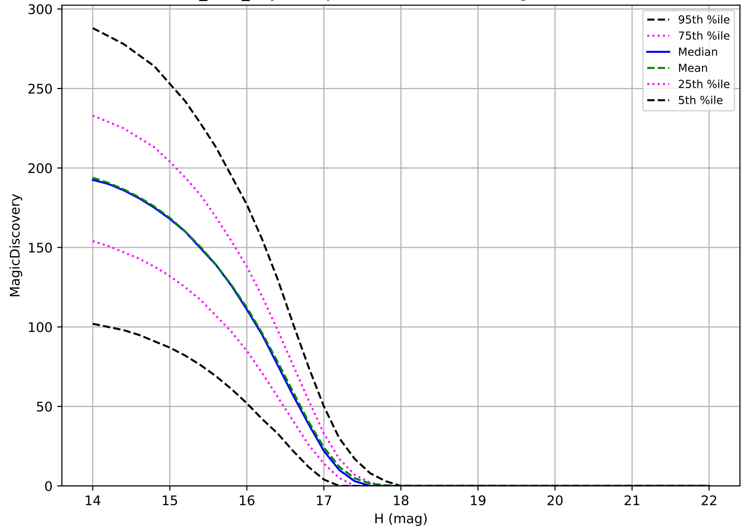
baseline_v3.3_10yrs: Trojan 6 detections in 60 nights detection loss
