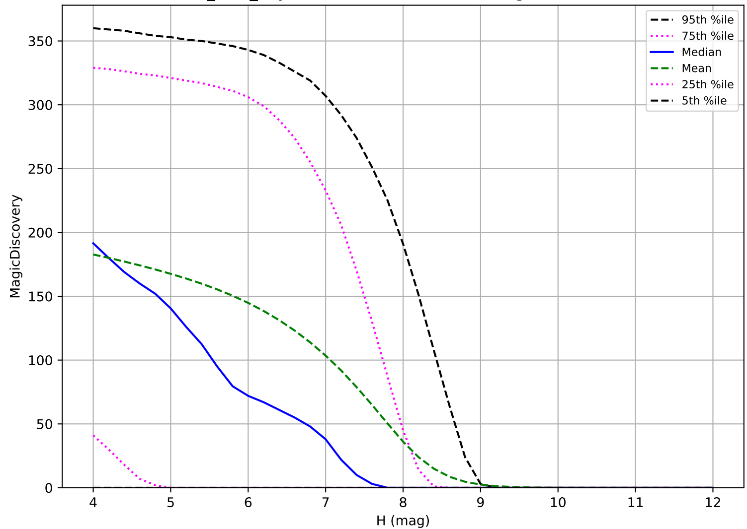
baseline_v3.3_10yrs: TNO 6 detections in 60 nights detection loss
