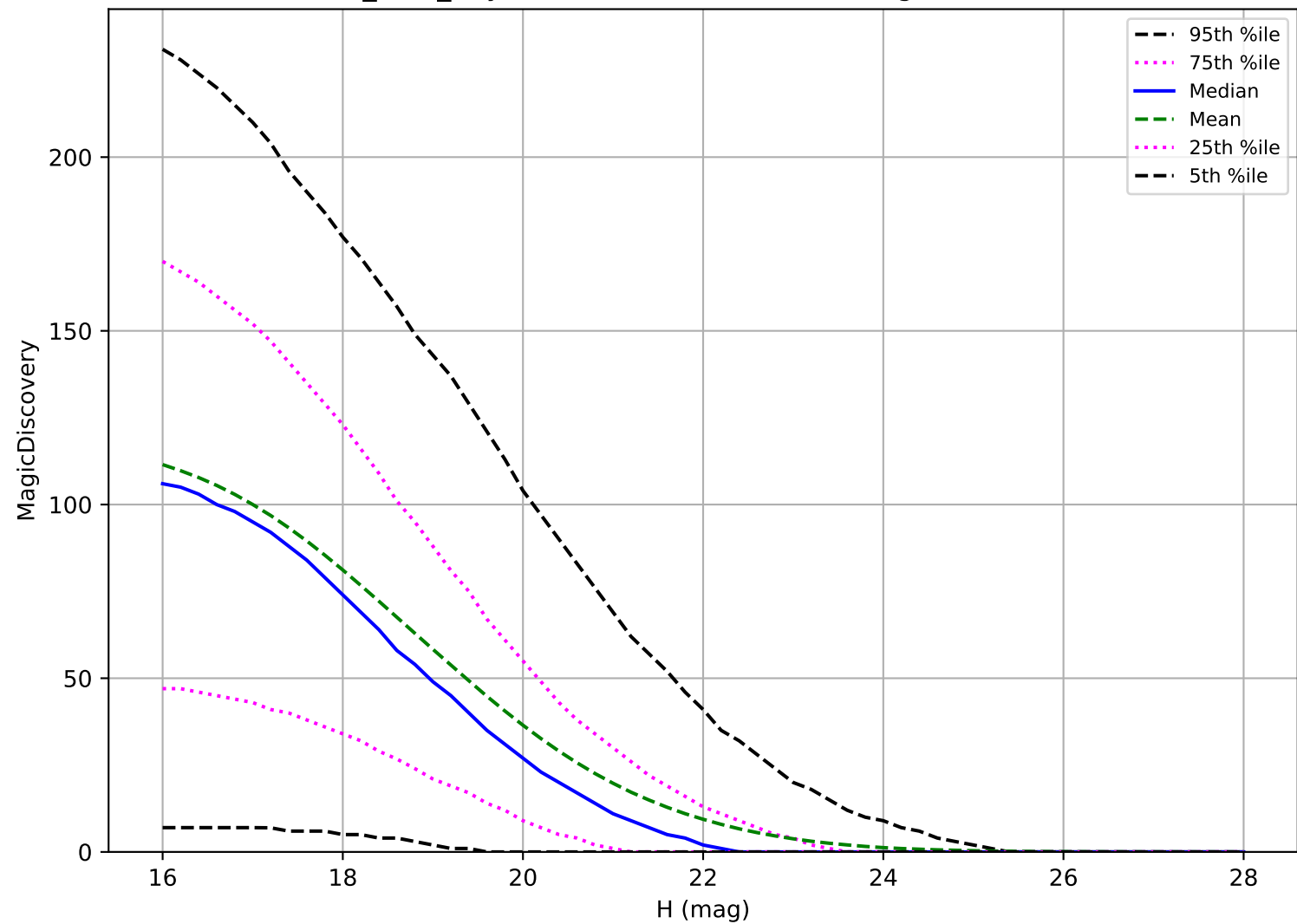
baseline_v3.3_10yrs: PHA 6 detections in 60 nights detection loss
