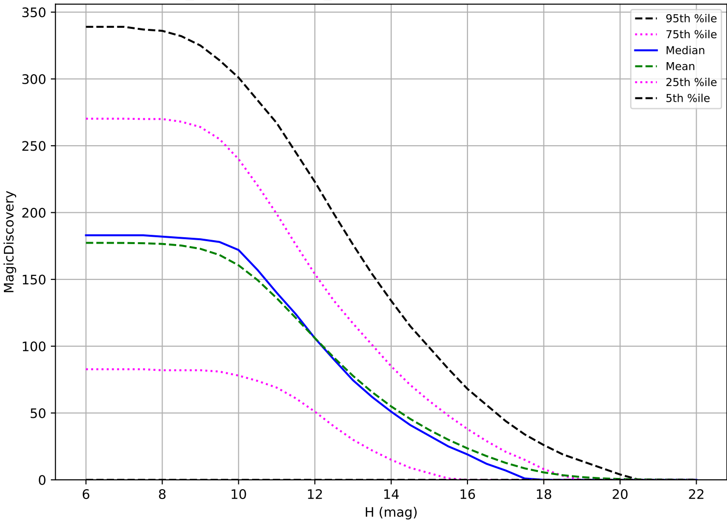
baseline_v3.3_10yrs: OCC_r5 6 detections in 60 nights detection loss
