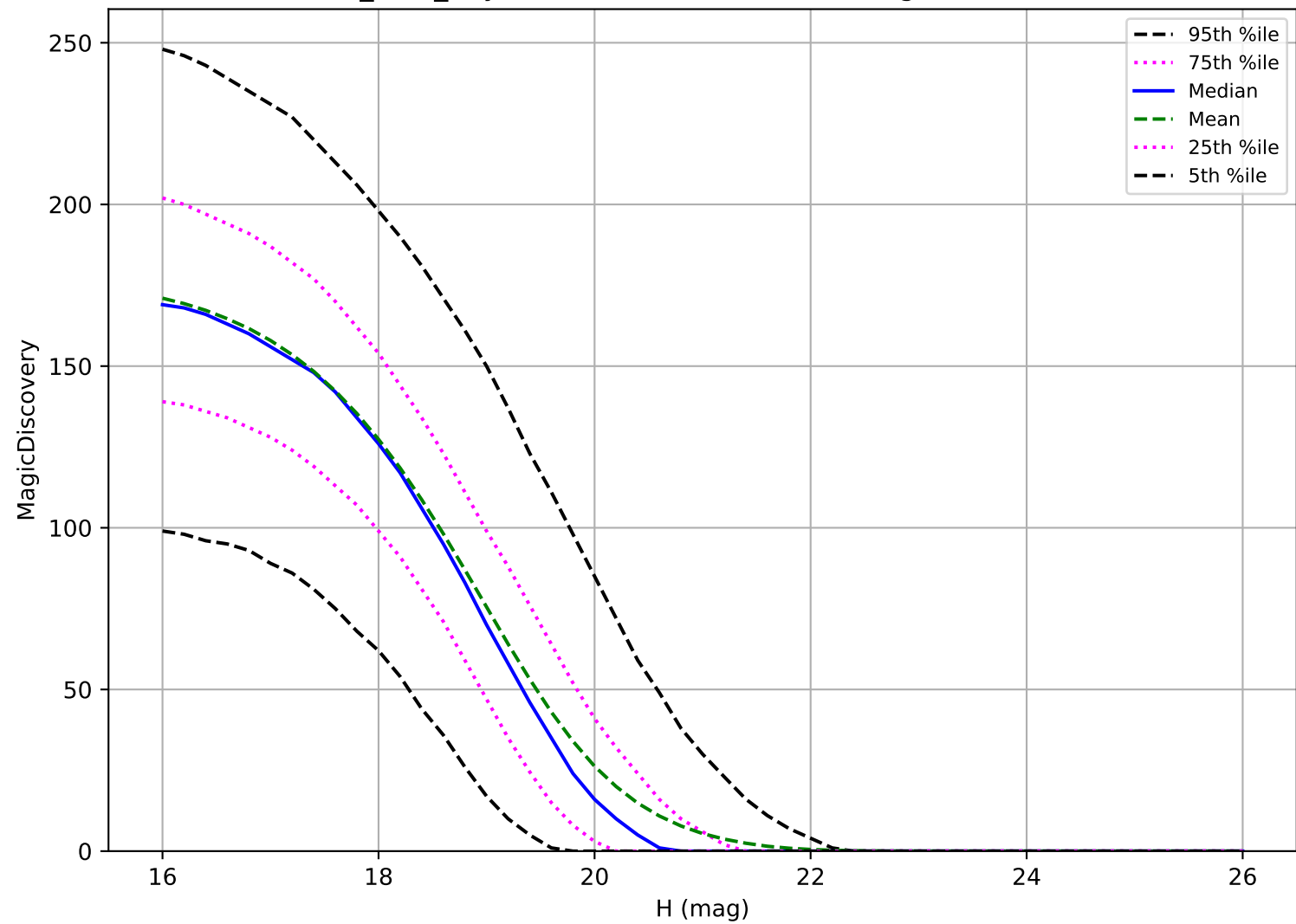
baseline_v3.3_10yrs: MBA 6 detections in 60 nights detection loss
