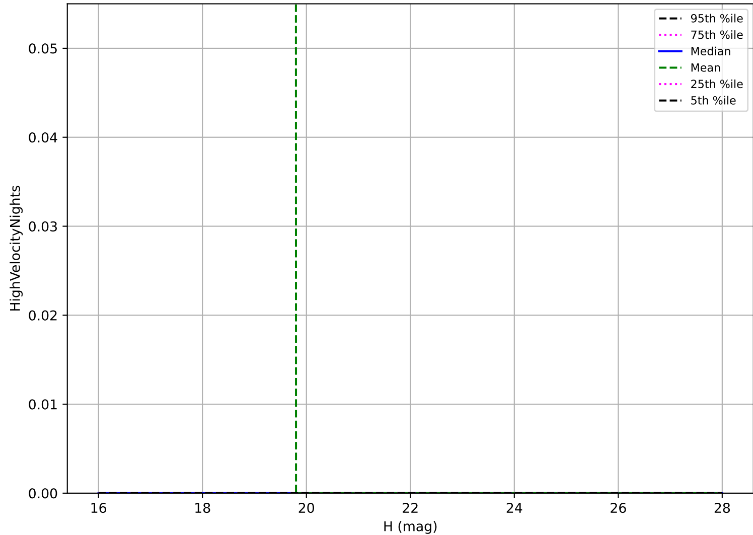
baseline_v3.3_10yrs: Vatira High velocity pair detection loss
