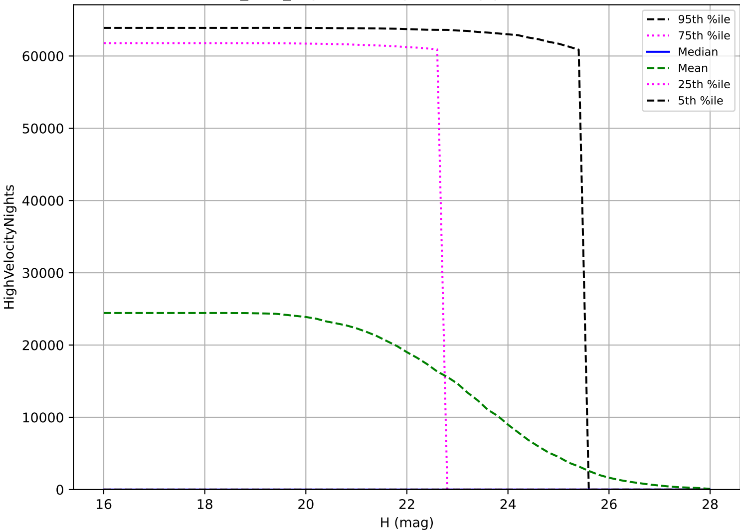
baseline_v3.3_10yrs: PHA High velocity pair detection loss
