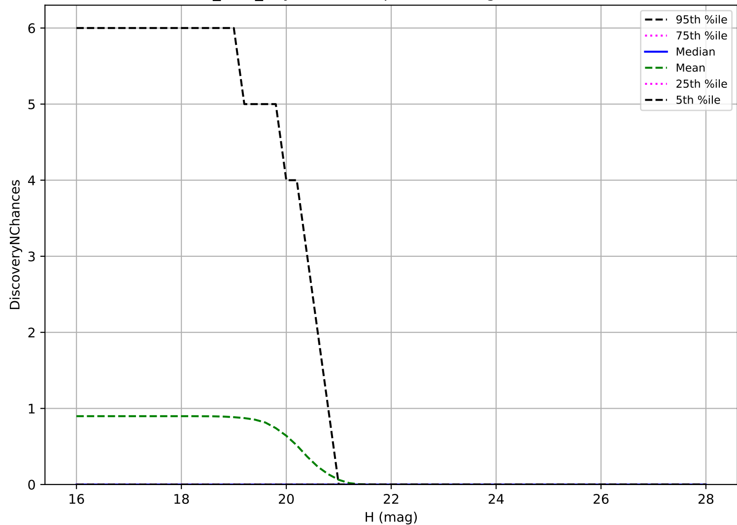
baseline_v3.3_10yrs: Vatira 3 pairs in 15 nights detection loss
