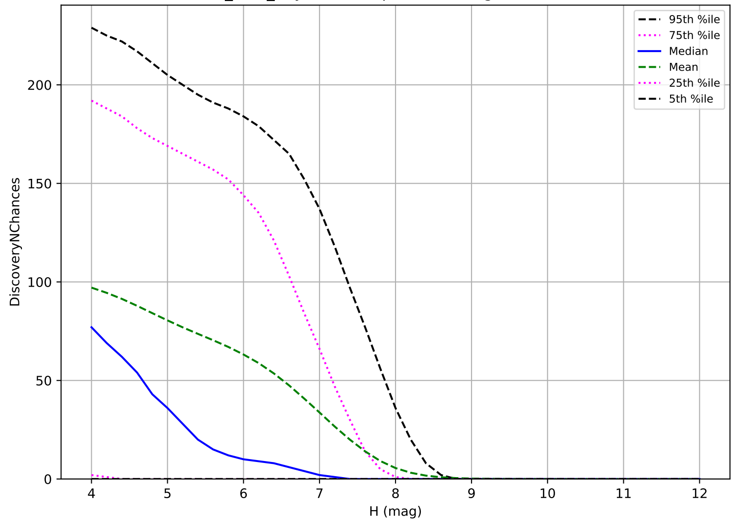
baseline_v3.3_10yrs: TNO 3 pairs in 15 nights detection loss
