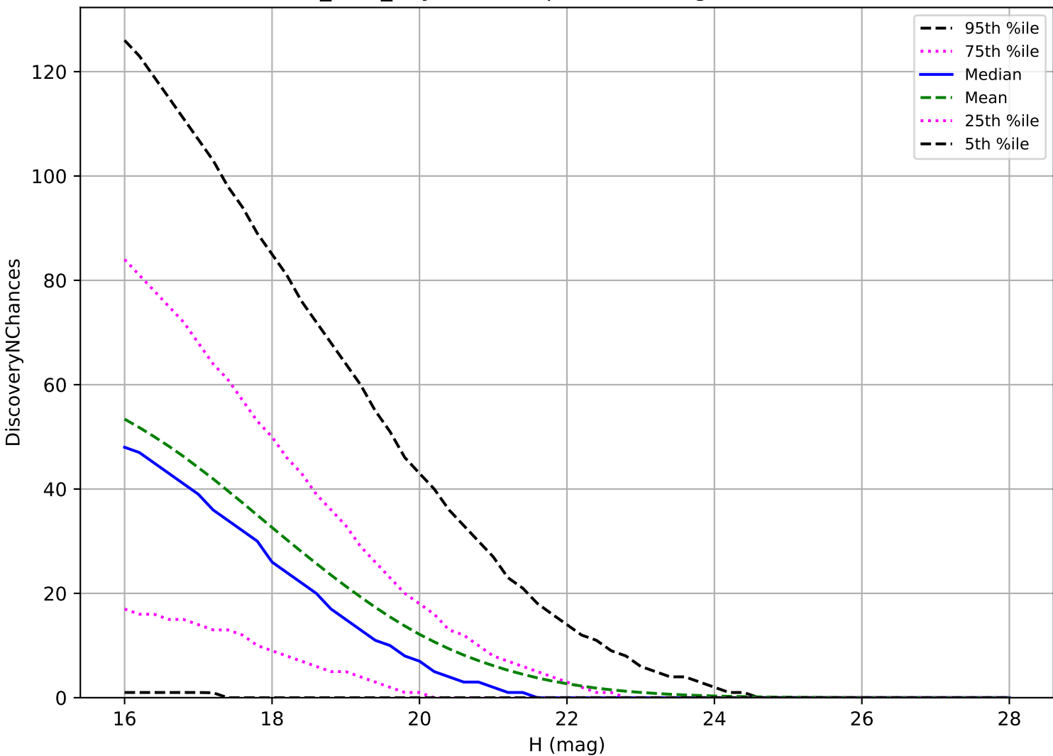
baseline_v3.3_10yrs: PHA 3 pairs in 15 nights detection loss
