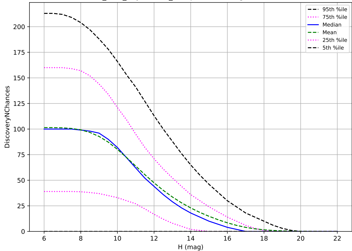
baseline_v3.3_10yrs: OCC_r5 3 pairs in 15 nights detection loss
